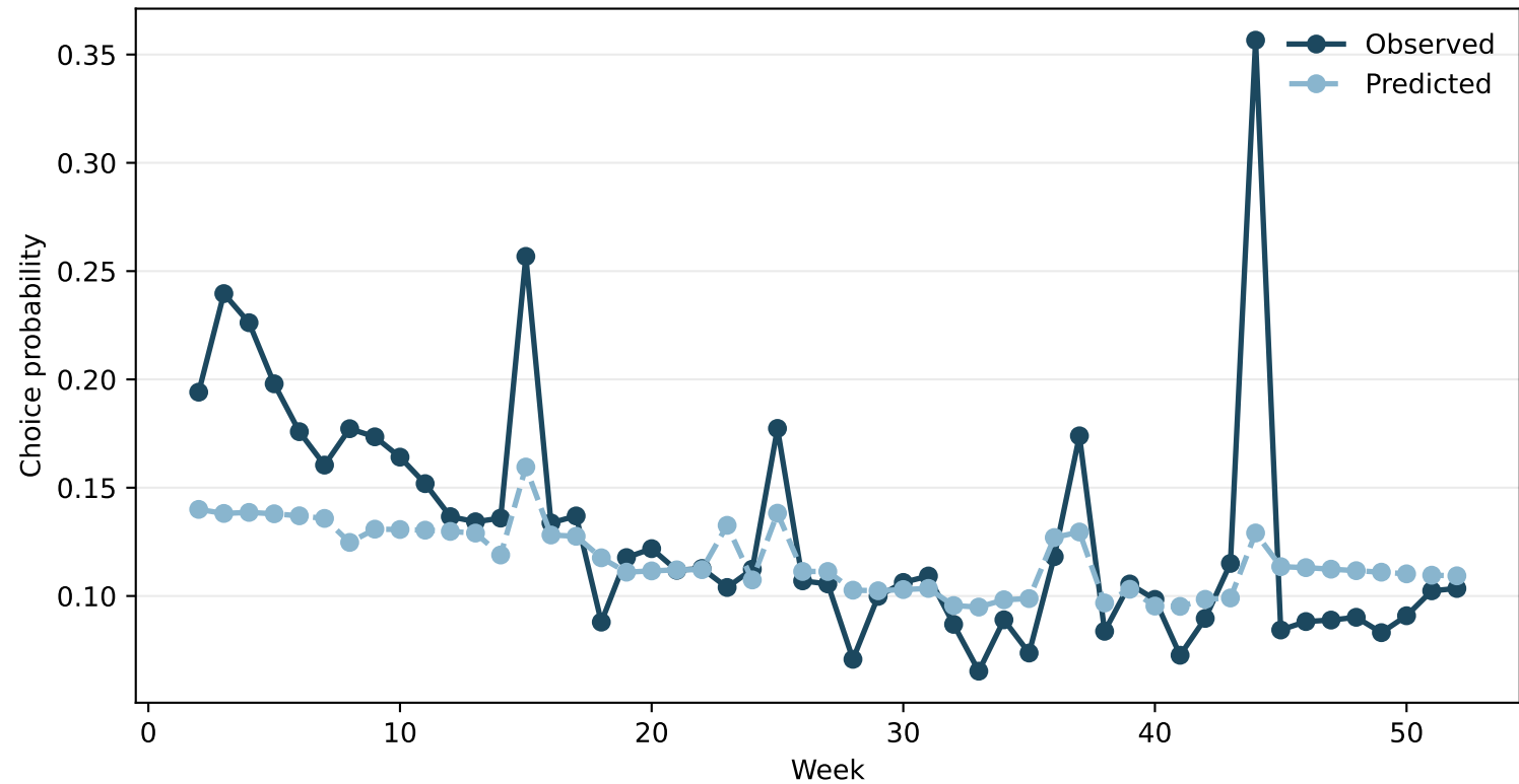
Observed vs. predicted choice probability: Navito
